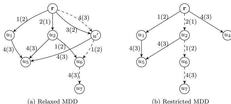
Fig. 2: A relaxed and a restricted MDD for the example instance in Fig. 1.
