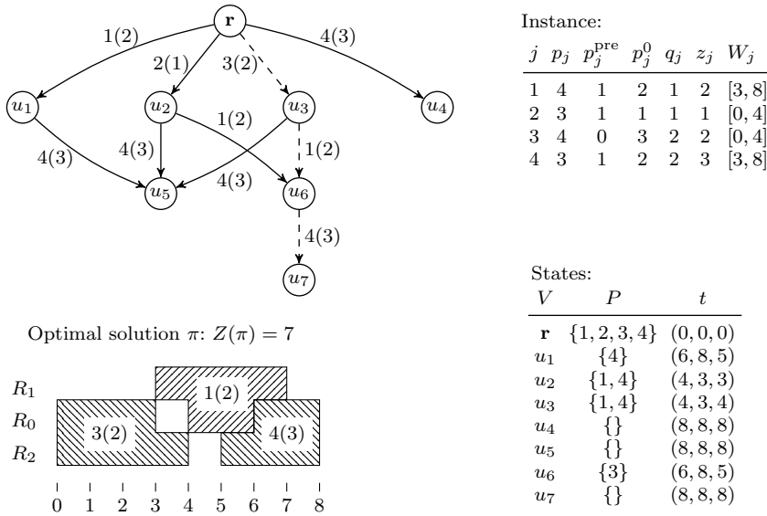
Fig. 1: A MDD for an example instance with four jobs and two secondary resources.
